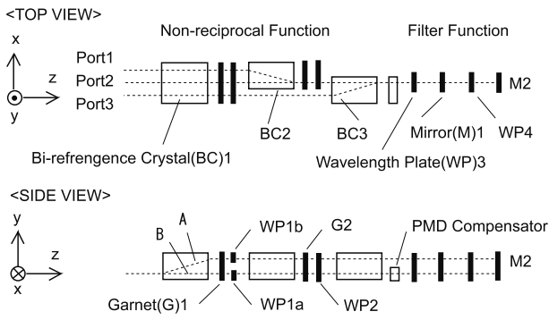
Fig. 2: Sustructure of new interleaver.
